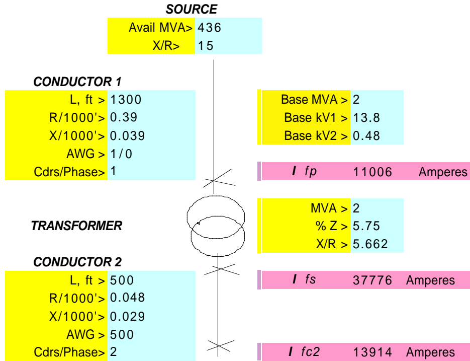
Figure B.1—Example—Part of bolted fault tab
