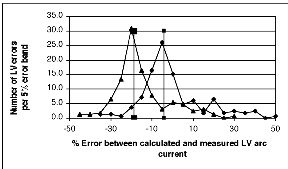
Figure 10—Histogram of LV arc current calculation error
