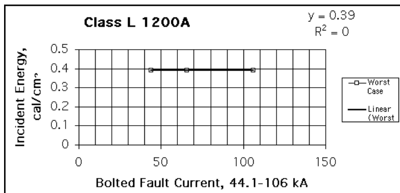
Figure E.12—Class L 1200 A fuse—upper current segment of model
