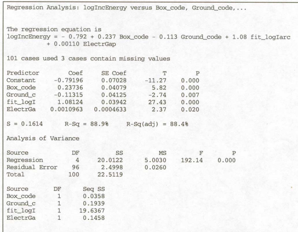
Figure 14—Program output 3— E_n regression analysis
